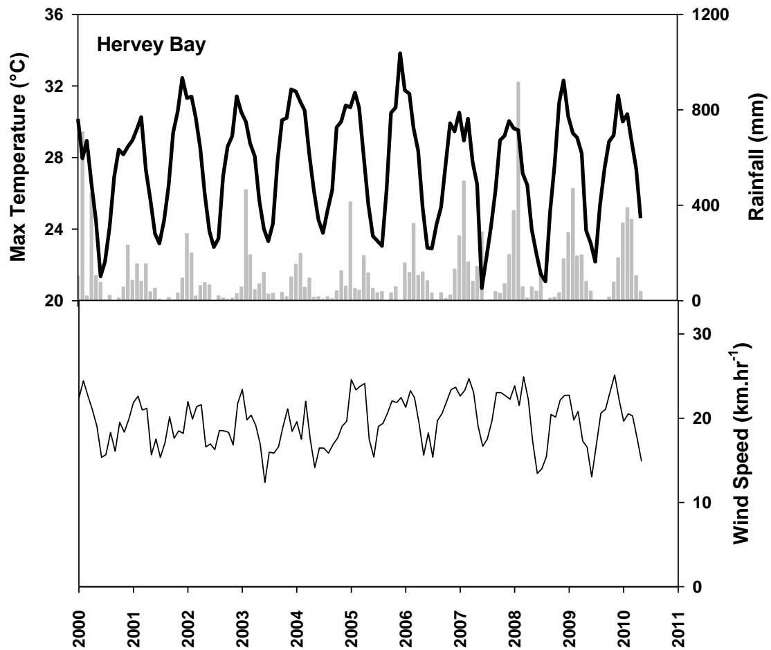
Figure 131. Mean monthly daily maximum temperature (°C), total monthly rainfall, mean monthly cloud cover (quarts), and mean monthly 3pm wind speed (km.hr -1 ) recorded at Hervey Bay Airport (BOM station 040405) (Source www.bom.gov.au ). Hervey Bay airport used as a surrogate for the climate at Urangan.
