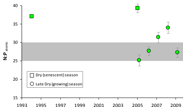
Figure 134. Elemental ratios (atomic) of seagrass leaf tissue N:P reported from Luggier Bay in July 1994 (Mellors 2003) and the present monitoring program (mean \pm Standard Error). Horizontal shaded band on the N:P ratio panel represents the range of value associated with N:P balance ratio in the plant tissues, i.e. a seagrass “Redfield” ratio (Atkinson and Smith, 1983; Duarte, 1990; Fourqurean et al. , 1992; Fourqurean & Cai 2001). N:P ratio above this band indicates P limitation and below indicates N limitation.
