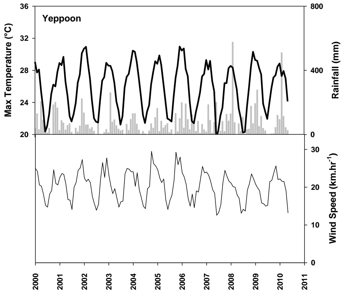
Figure 115. Mean monthly daily maximum temperature (°C), total monthly rainfall, mean monthly cloud cover (quarts), and mean monthly 3pm wind speed (km.hr -1 ) recorded at Yeppoon (BOM station 033106) (Source www.bom.gov.au ). Yeppoon used as a surrogate for the climate at Great Keppel Island and Shoalwater Bay
