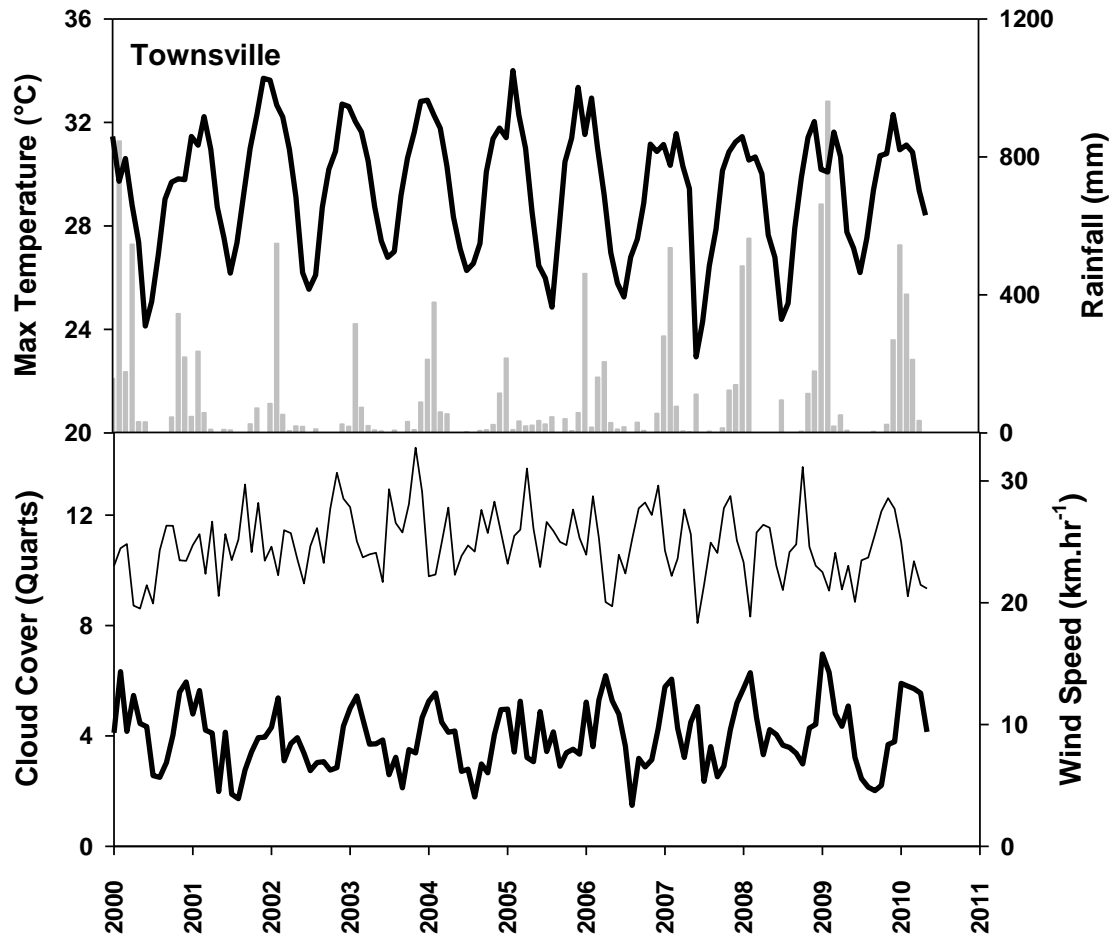
Figure 68. Mean monthly daily maximum temperature (°C), total monthly rainfall, mean monthly cloud cover (quarts), and mean monthly 3pm wind speed (km.hr -1 ) recorded at Townsville Airport (BOM station 032040) (Source www.bom.gov.au ). Townsville Airport used as a surrogate for the climate at coastal (Townsville) and reef (Magnetic Island) locations.
