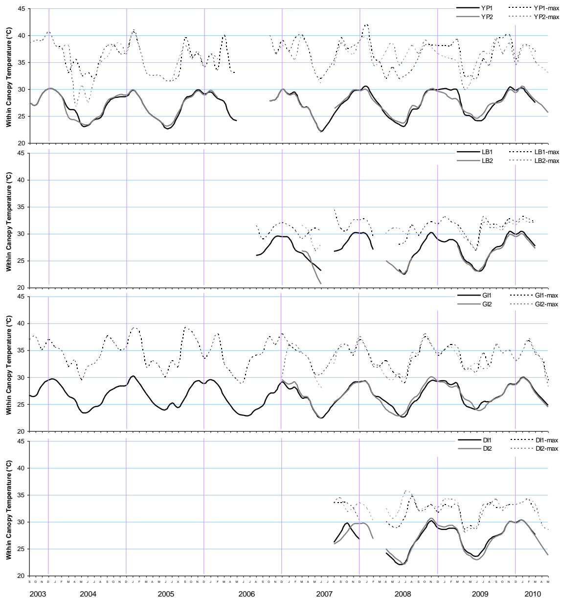
Figure 45. Monthly mean and maximum within seagrass canopy temperatures (°C) at coastal (Yule Point and Luggar Bay) and fringing-reef (Green Island and Dunk Island) intertidal meadows within the Wet Tropics region.
