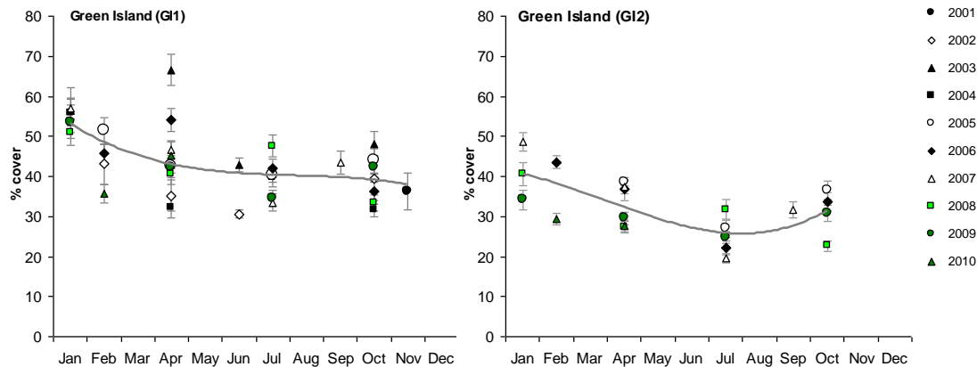
Figure 32. Mean percentage seagrass cover (all species pooled) ( \pm Standard Error) at Green Island long-term monitoring sites at time of year. NB: Polynomial trendline for all years pooled.
