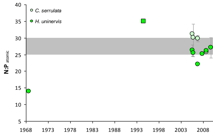
Figure 137. Elemental ratios (atomic) of seagrass leaf tissue N:P reported from Cackle Bay (Magnetic Island) in 1968 (Brich 1975), July 1994 (Mellors 2003) and the present monitoring program (mean \pm Standard Error). Horizontal shaded band represents the range of value associated with N:P balance ratio in the plant tissues, i.e. a seagrass “Redfield” ratio. N:P ratio above this band indicates P limitation and below indicates N limitation. Square symbol illustrates samples from the senescent season.
