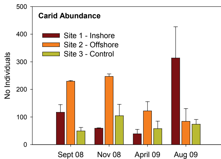
Figure 10. Mean number of caridean shrimp \pm SE at the three beam trawl survey sites (Inshore, Offshore & Control) surveyed between September 2008 and August 2009.
