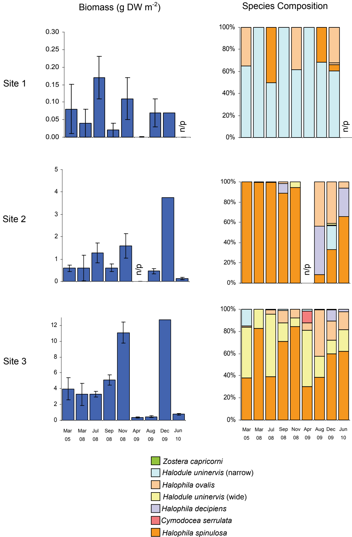
Figure 3. Changes in Meadow biomass, area and species composition for the deepwater seagrass monitoring sites in the Port of Abbot Point, March 2005 & February/March 2008 – June 2010
